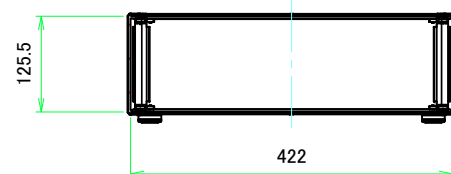
B-B (1:7)
