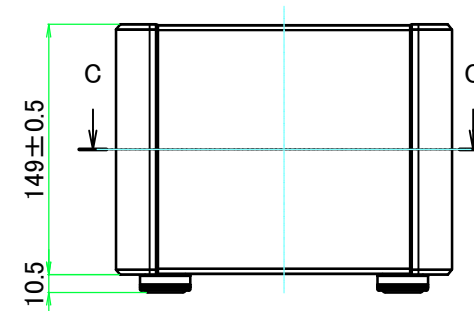
A view
