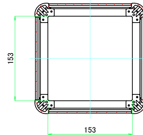
C-C (1:4)
