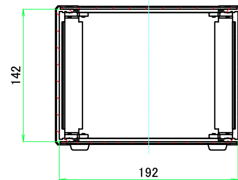
B-B (1:4)
