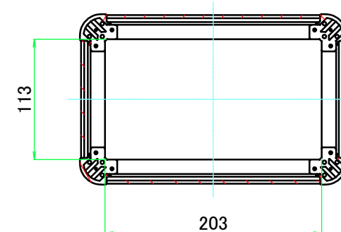
C-C (1:5)
