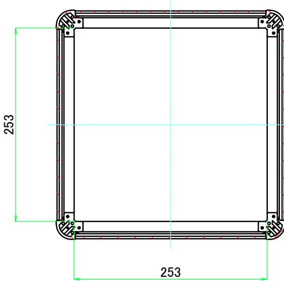
C-C (1:5)
