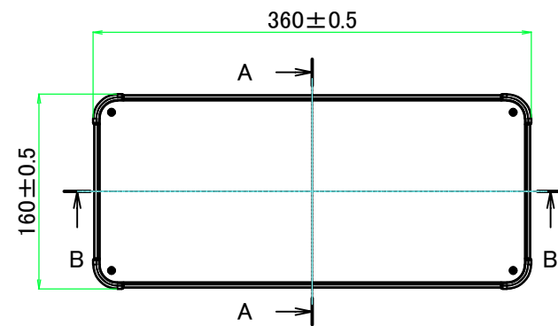
E view
