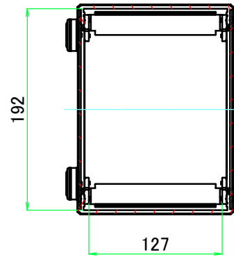
B-B (1:5)
