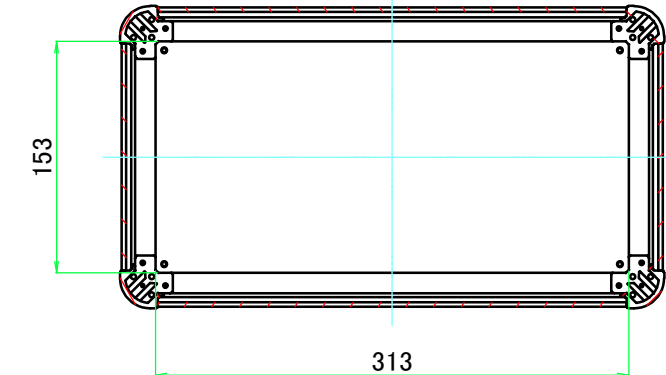
C-C (1:5)
