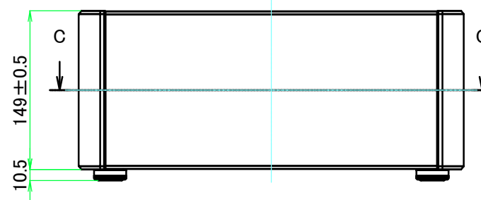
A view
