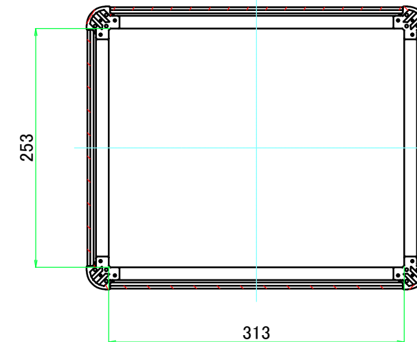
C-C (1:5.5)
