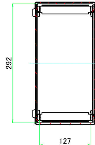
A-A (1:5.5)
