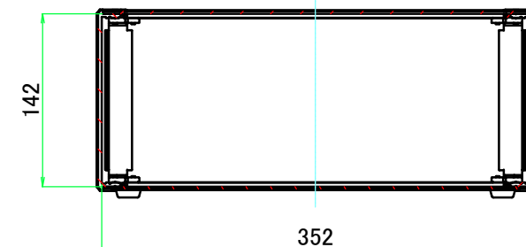
B-B (1:5.5)
