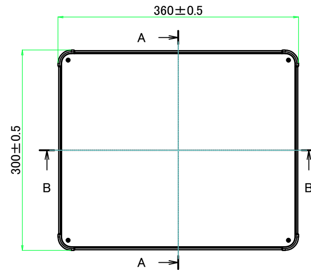
E view
