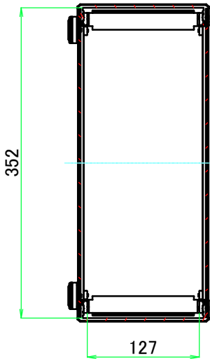
B-B (1:6)
