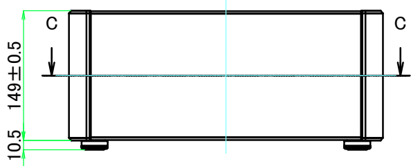
A view
