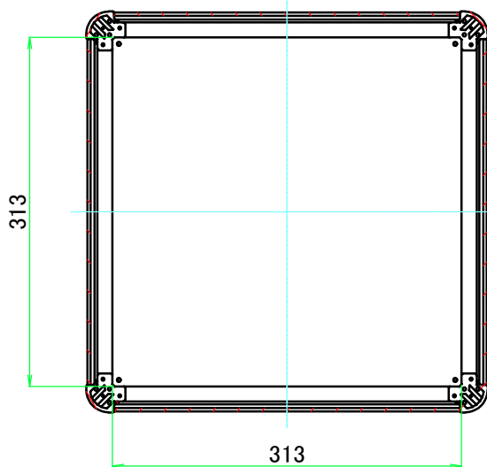
C-C (1:6)
