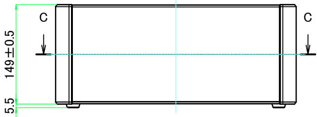
A view
