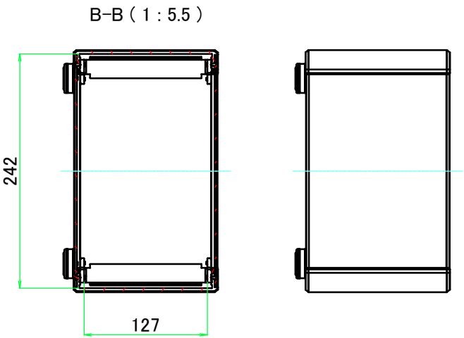
D view
