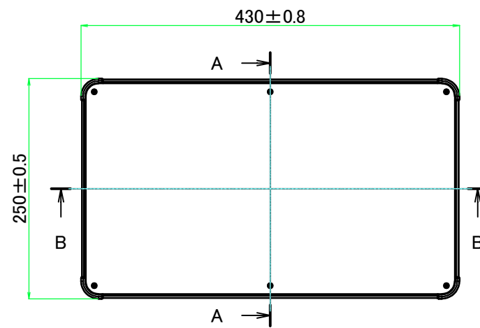
E view
