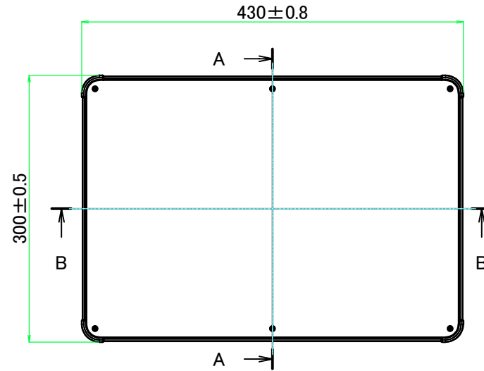
E view
