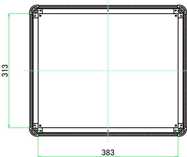
C-C (1:6.5)
