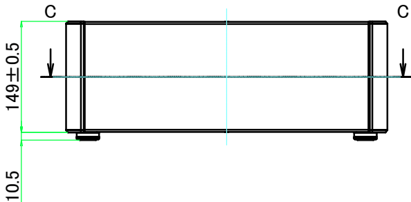
A view
