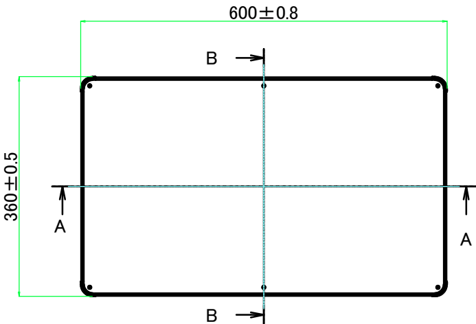
E view
