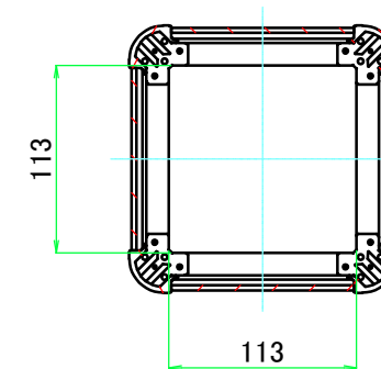
C-C (1:5)
