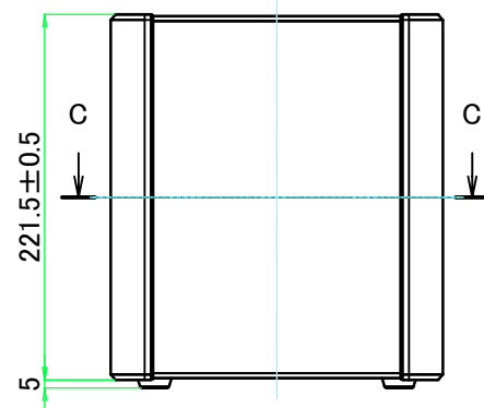
A view
