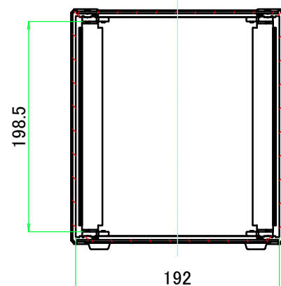
B-B (1:5)
