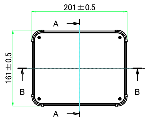
E view
