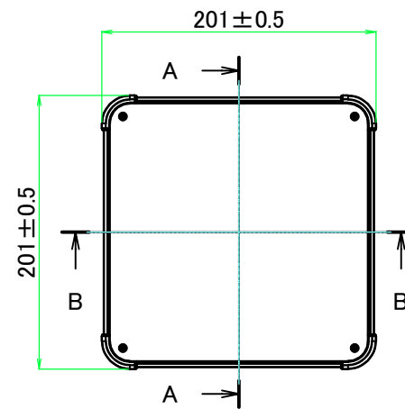
E view
