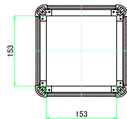
C-C (1:5)
