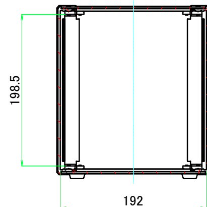
B-B (1:5)
