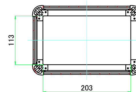
C-C (1:5)
