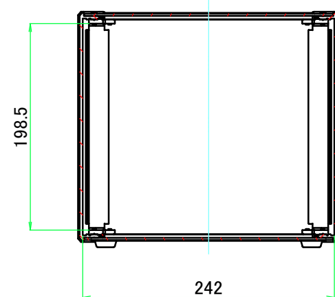
B-B (1:5)
