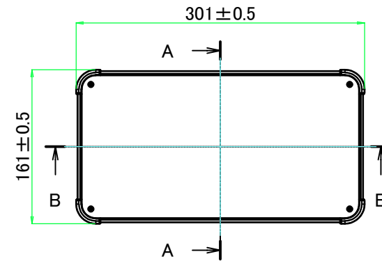
E view
