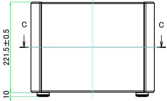
A view
