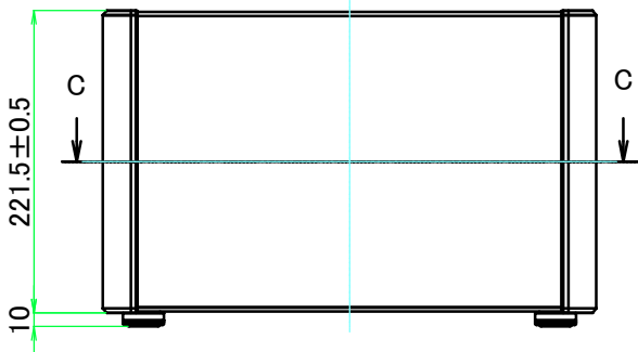
A view
