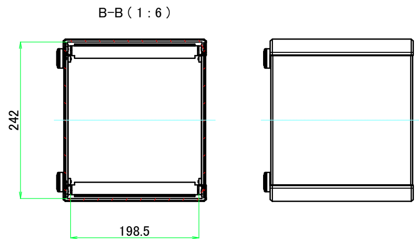
D view
