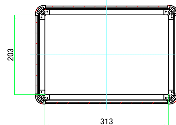
C-C (1:6)
