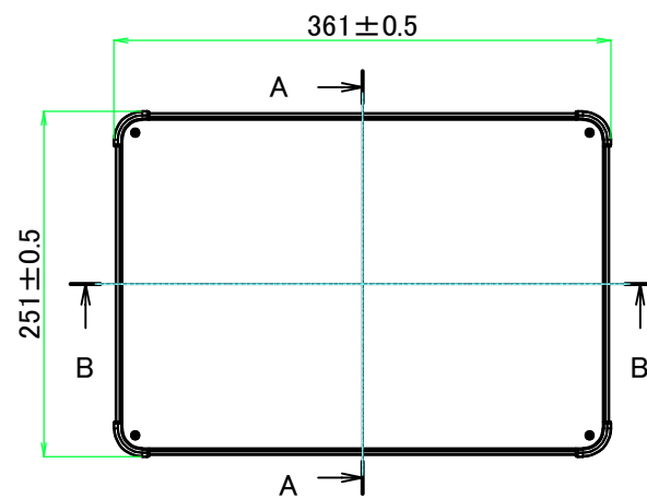
E view
