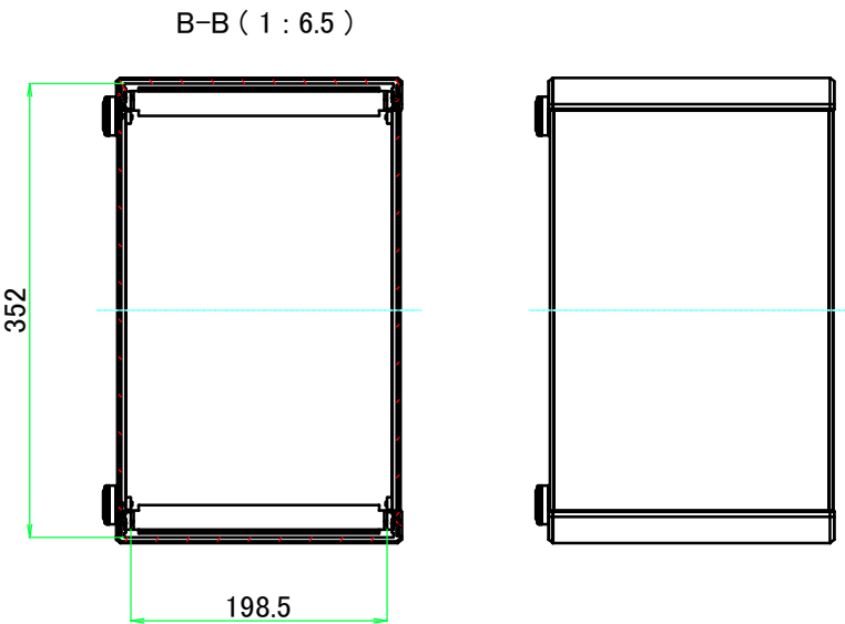
D view
