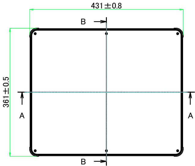
E view
