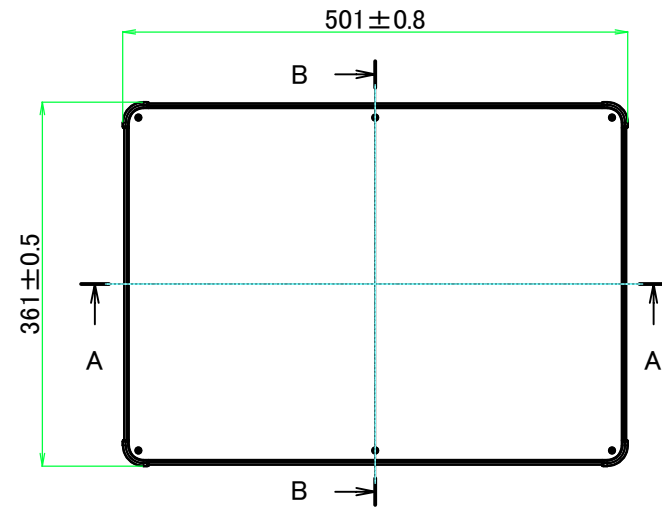
E view
