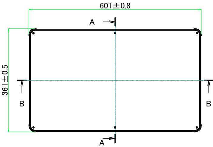
E view
