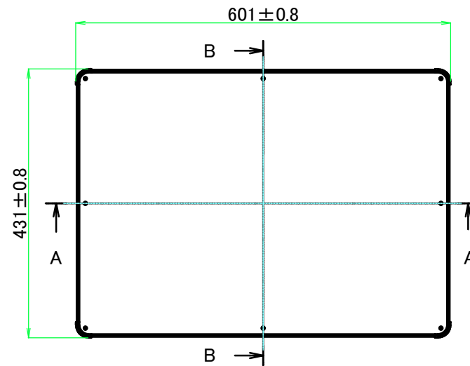
E view
