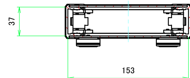
B-B (1:3)
