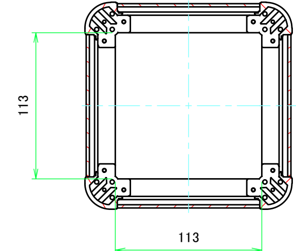
C-C (1:3)
