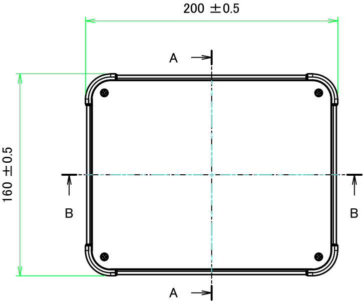
E view
