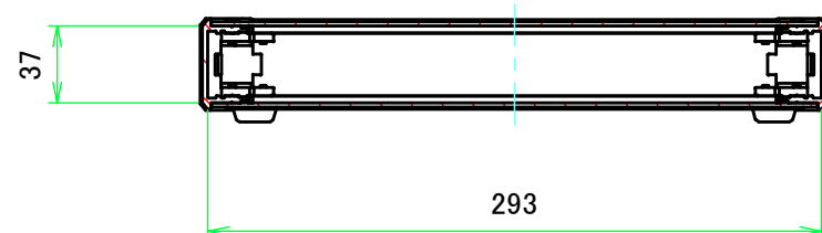
B-B (1:4)
