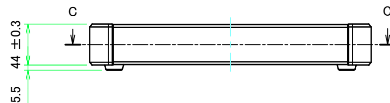
A view
