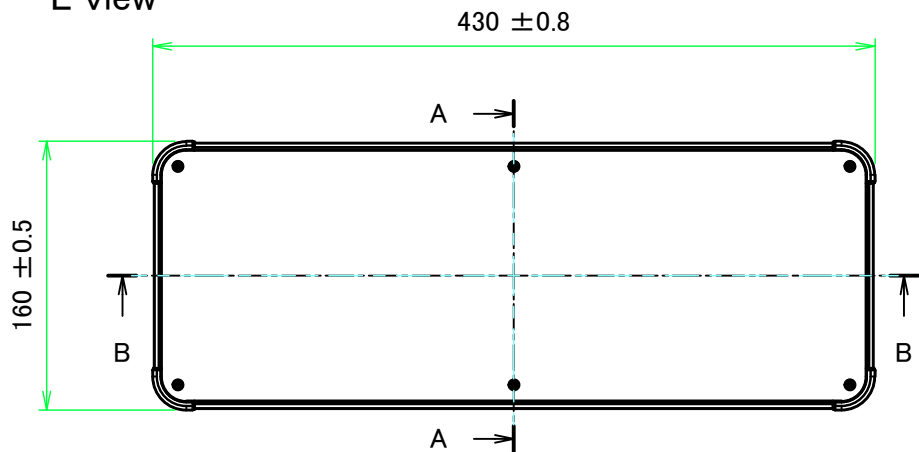
E view
