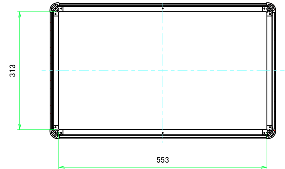
C-C (1:6)
