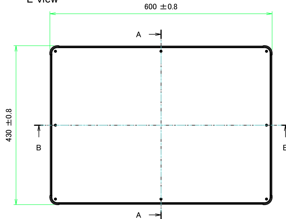
E view
