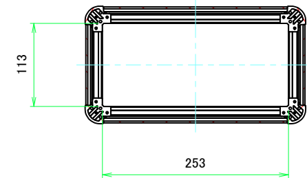
C-C (1:5)
