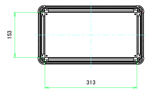
C-C (1:5.5)
