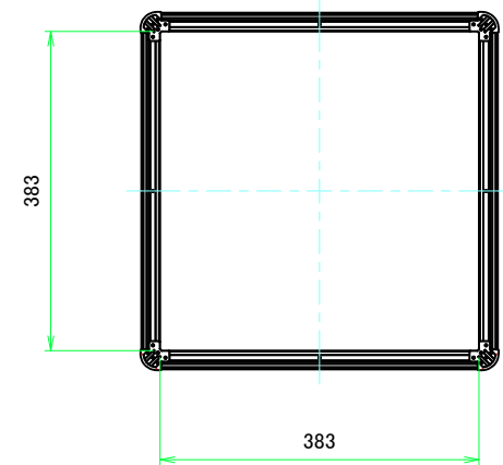
C-C (1:7)
