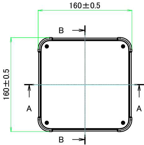
E view
