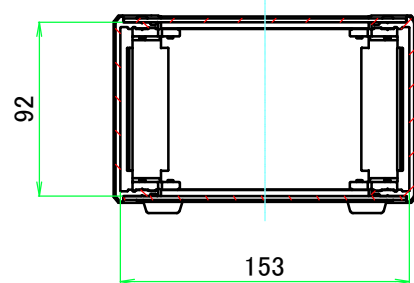
B-B (1:4)
