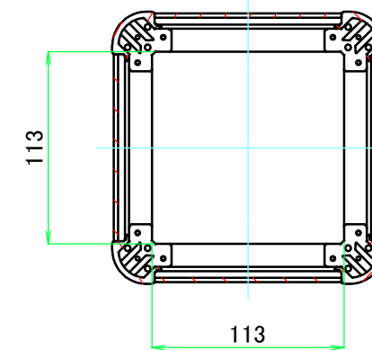
C-C (1:4)
