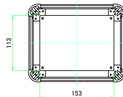
C-C (1:4)
