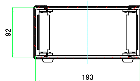
B-B (1:4)
