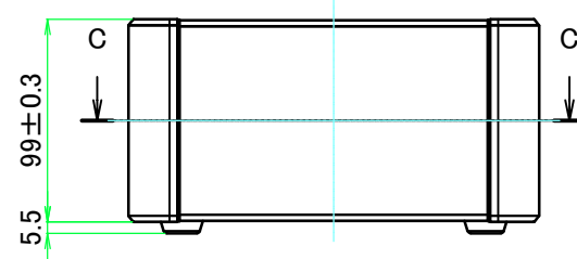
A view
