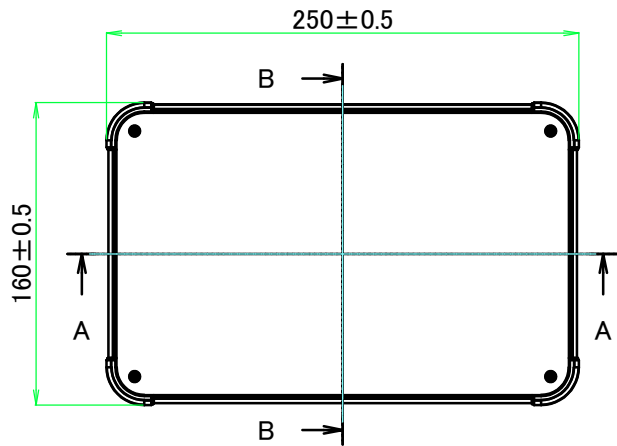
E view
