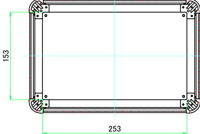
C-C (1:4)
