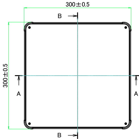
E view
