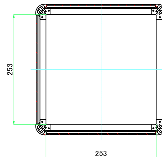
C-C (1:5)
