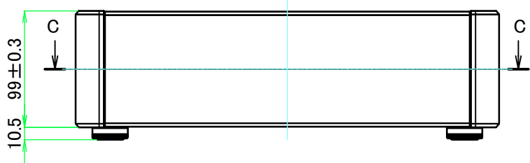
A view
