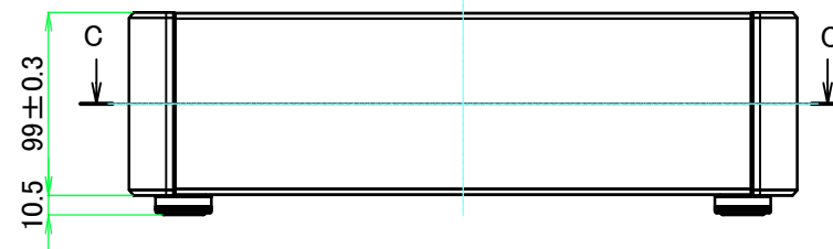
A view
