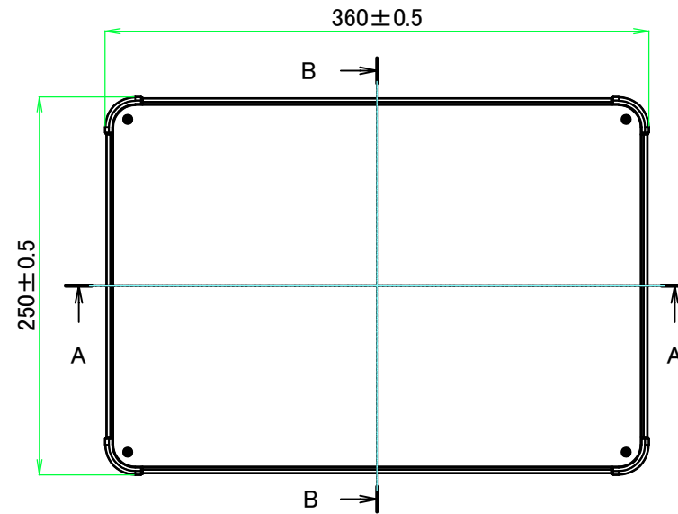
E view
